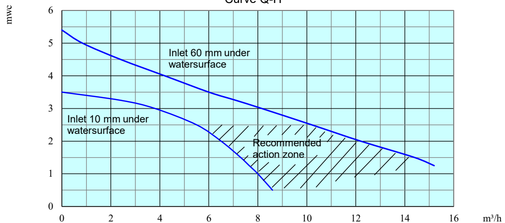
Curve Q-H
