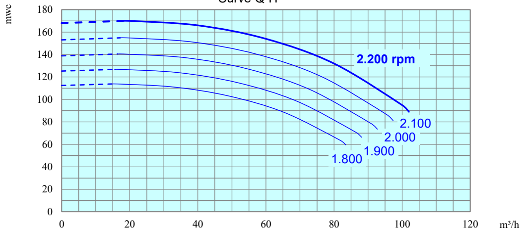
Curve Q-H
