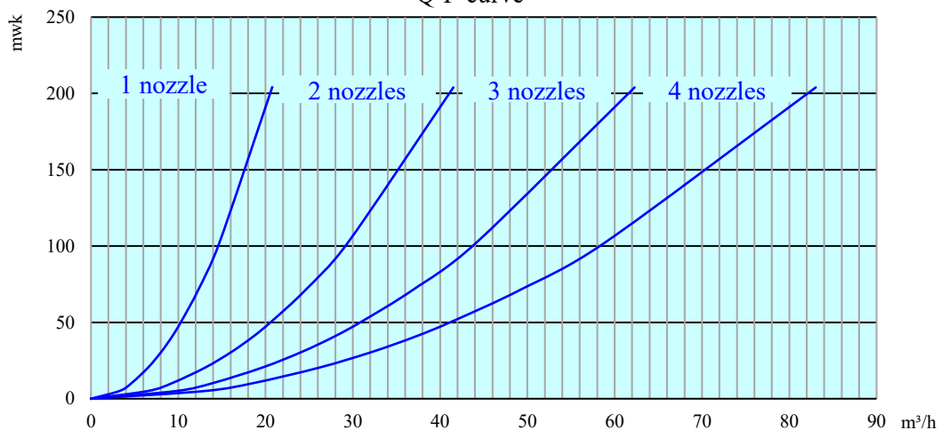
Q-P curve
