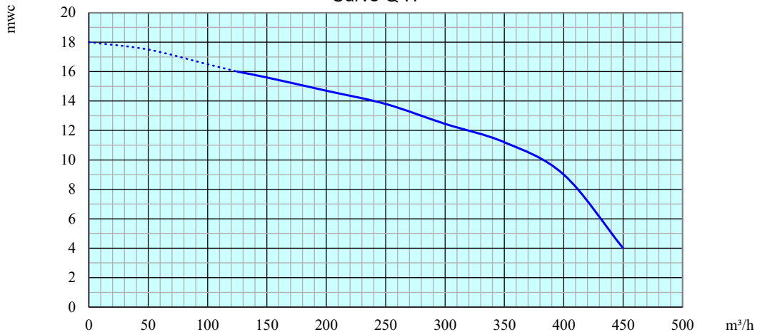
Curve Q-H
