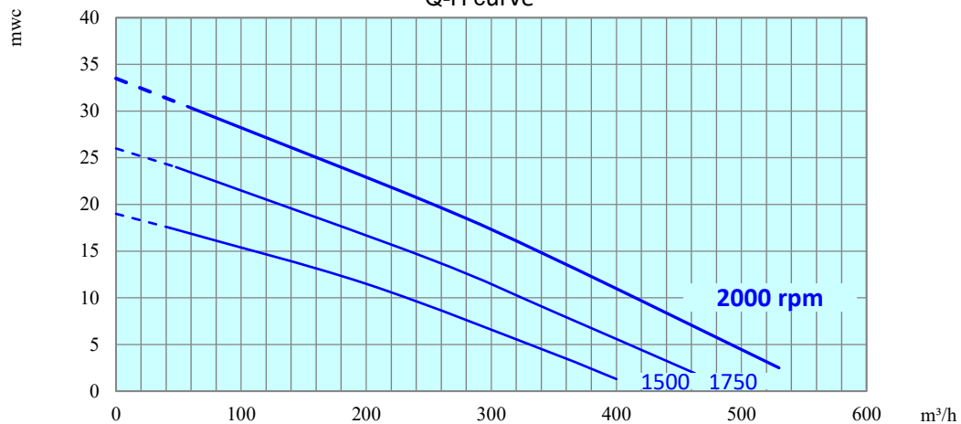
Q-H curve
