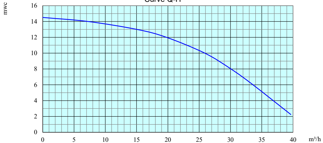
Curve Q-H
