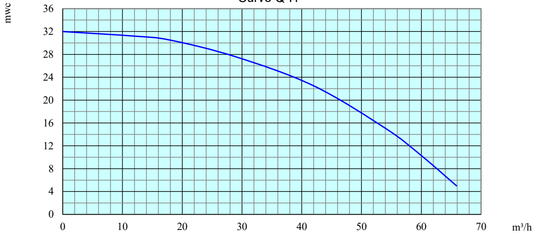
Curve Q-H
