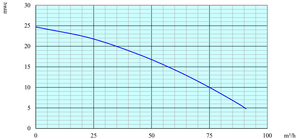
Curve Q-H
