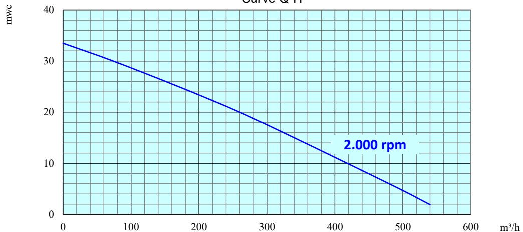
Curve Q-H
