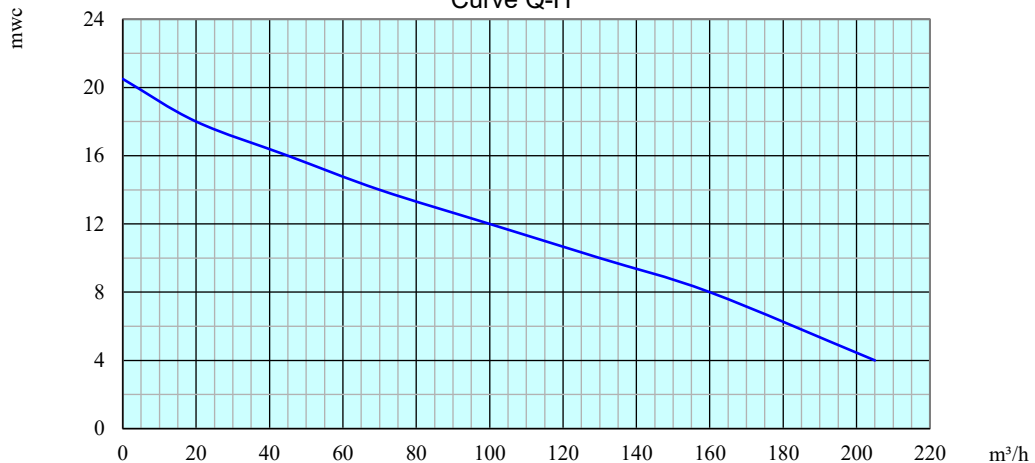
Curve Q-H
